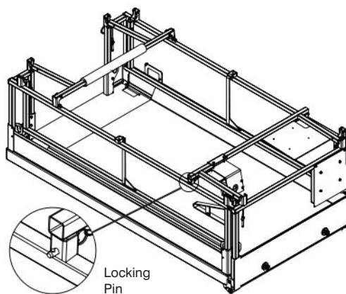
Figure 2-16b. All Guardrails Folded Down
