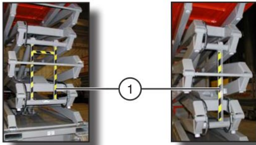
Figure 2-24. Maintenance Support
