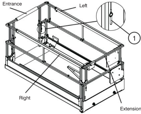
Figure 2-11. Folding Guardrail System
