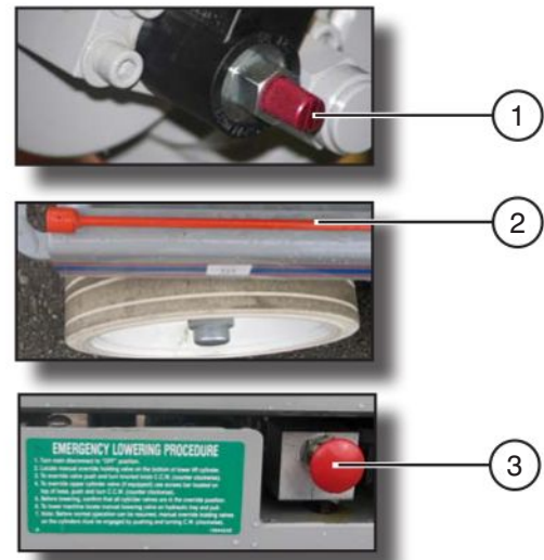
Figure 2-23. Emergency Lowering System
